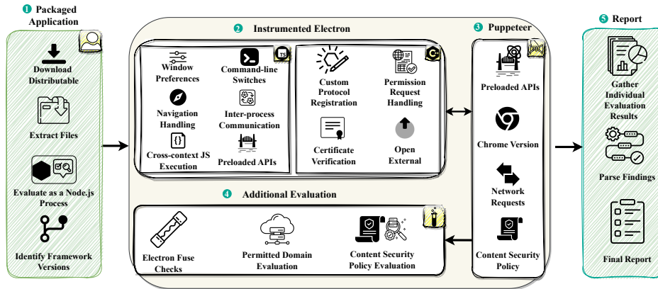
Figure 3: Inspector's components and auditing workflow for evaluating Electron apps.
