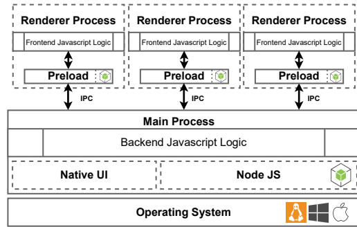
Figure 1: Architecture of Electron apps.
